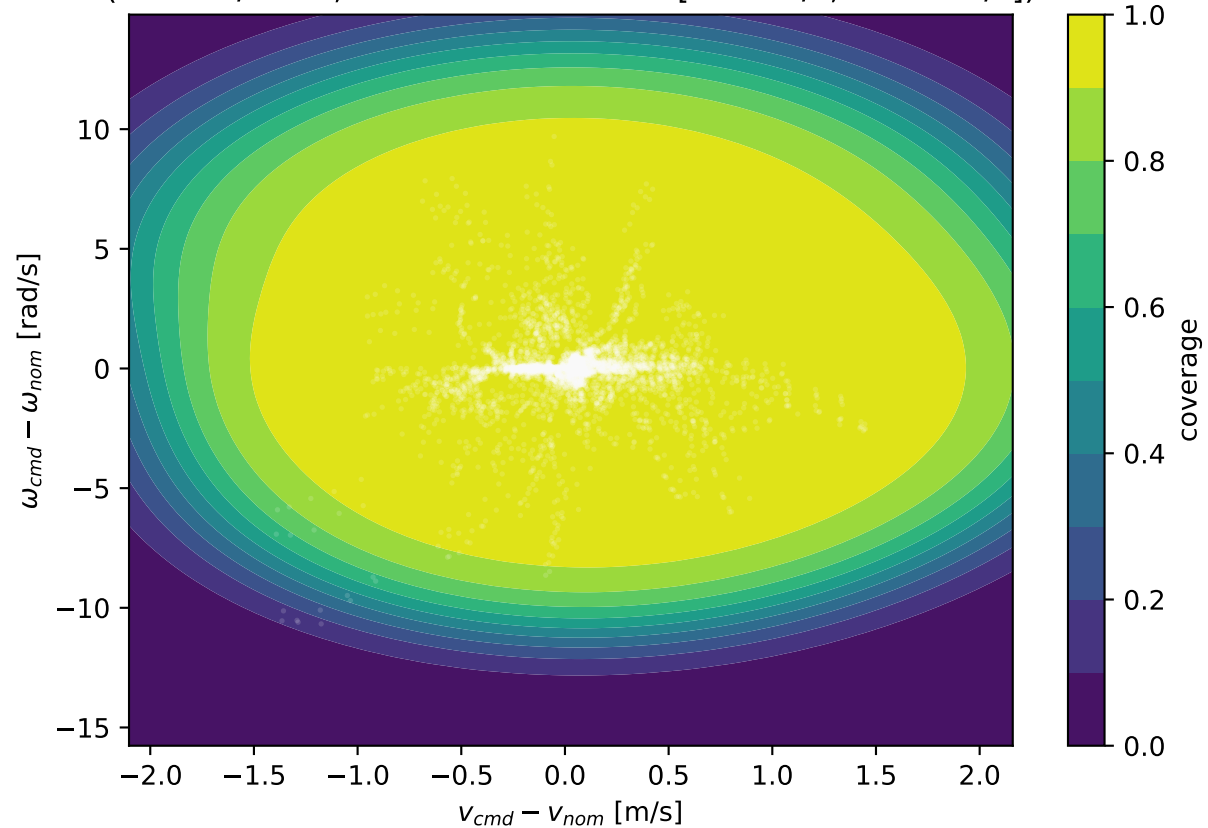
Residual coverage vs command offset (0 = off / OOD; state fixed at mean [0.54 m/s, 0.24 rad/s])
